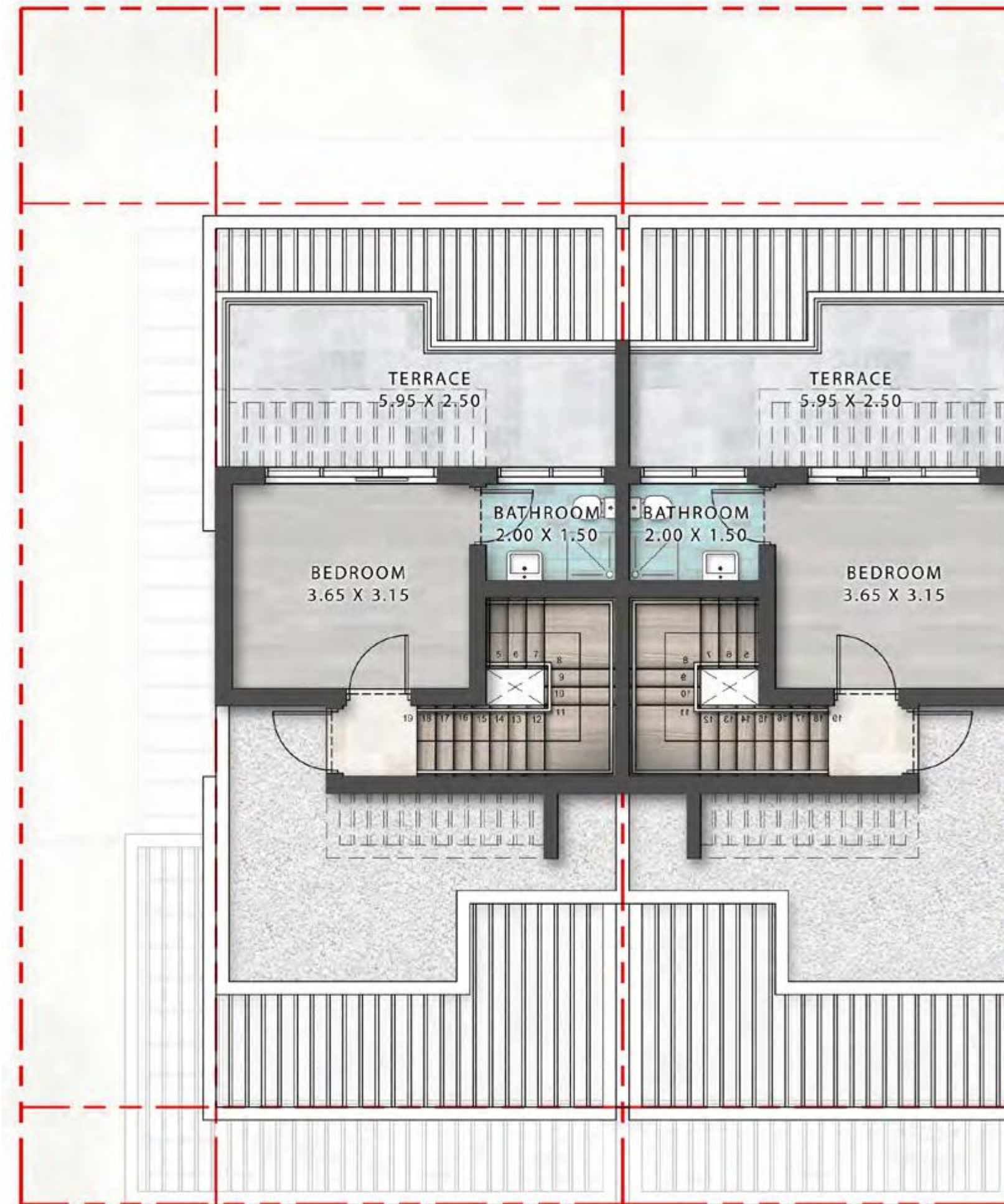
ROOF FLOOR (FUTURE EXPANSION)
